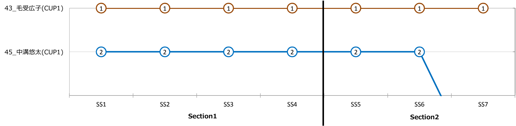
TRDCUP1Class _ AfterStageTotalTimeRankingChart
