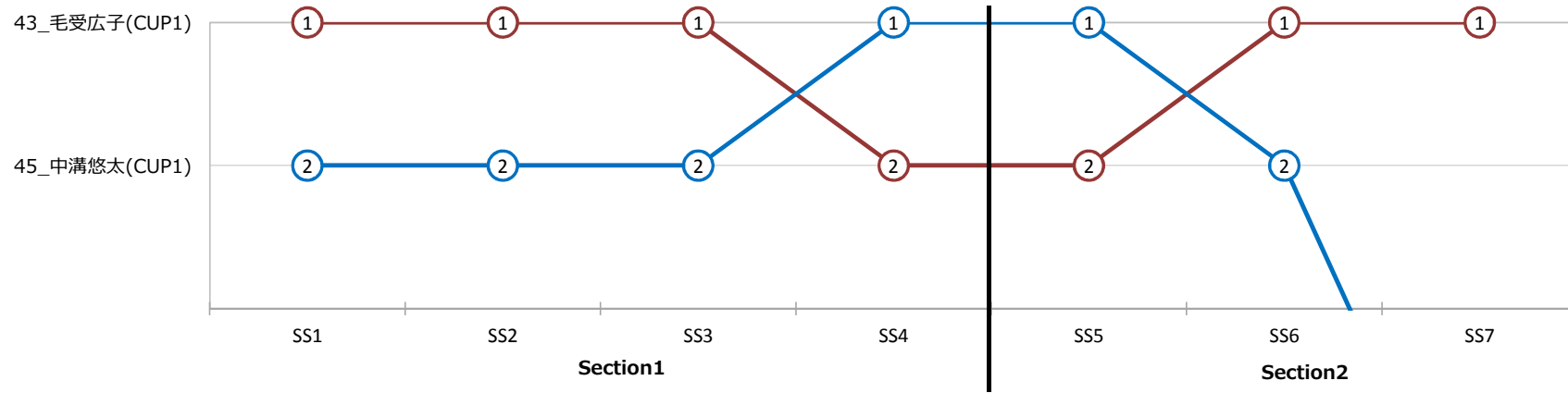
TRDCUP1Class _ StageTimeRankingChart
