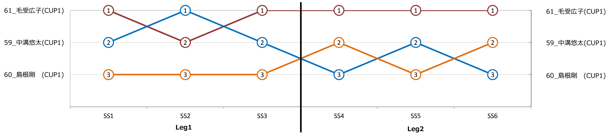
TRDCUP1Class _ StageTimeRankingChart
