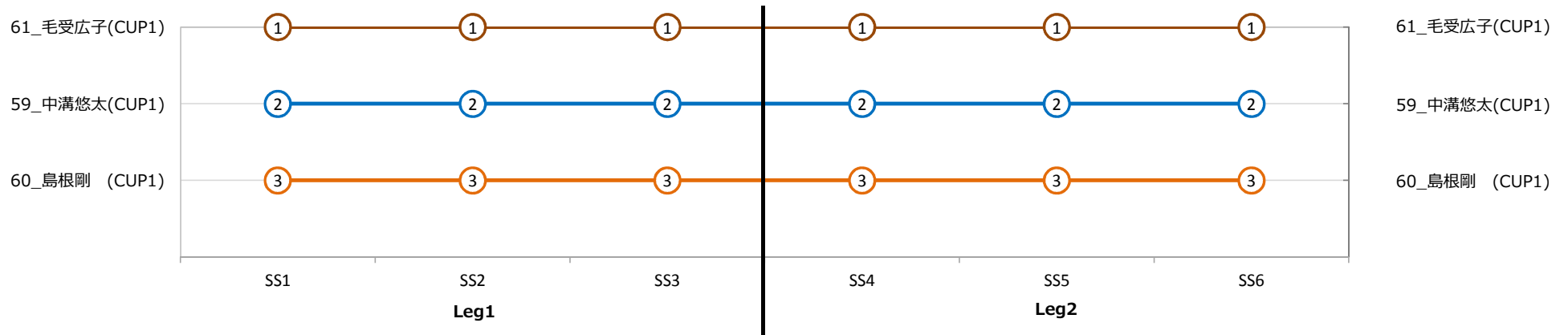
TRDCUP1Class _ AfterStageTotalTimeRankingChart
